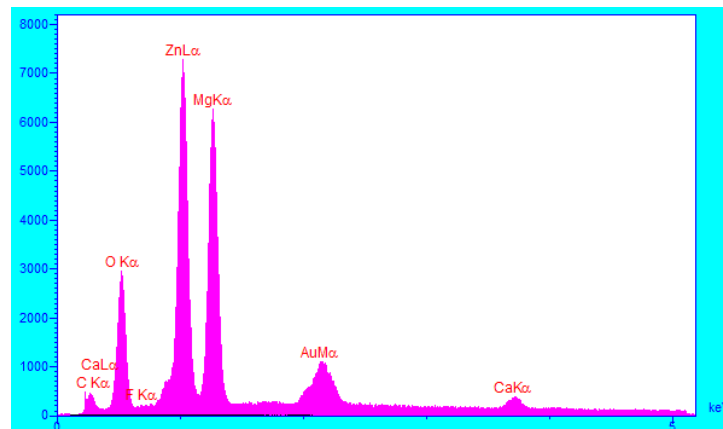
Fig. 4 EDS analysis of the synthesized Mg-4wt.% Zn scaffold
