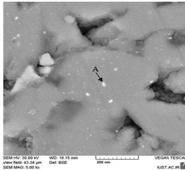
Fig. 3 SEM micrograph of the synthesized Mg-4wt.% Zn scaffold
