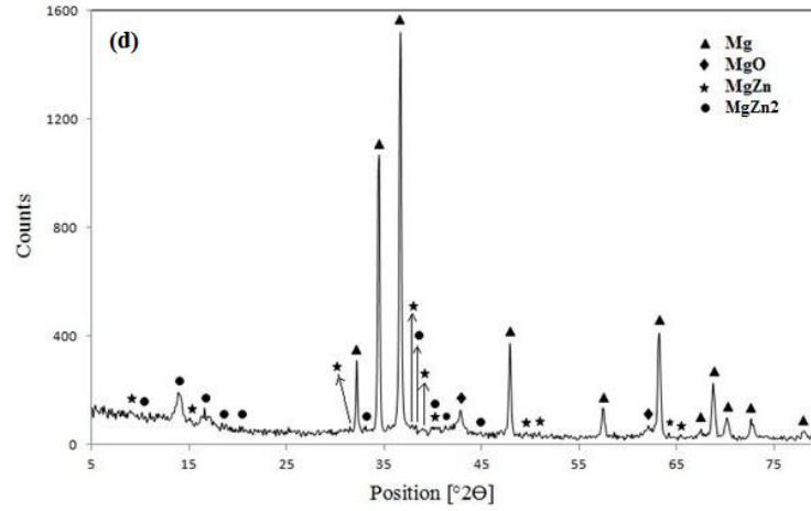
Fig. 2 The XRD patterns of the synthesized scaffolds containing different Zn amounts: (a) 1, (b) 2, (c) 3 and (d) 4 wt. %
