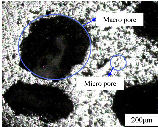
Fig. 1 The optical micrograph of the synthesized Mg-2wt.% Zn scaffold
