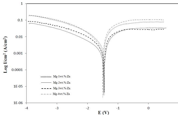
Fig. 5 Electrochemical polarization curves of the Mg-Zn scaffolds containing different Zn amounts
